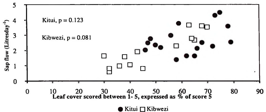
Figure 6.5.3.1.1 Trends of leaf cover and transpiration rates over same period for the Kitui and Kibwezi provenances in trial 1 at Machakos.
