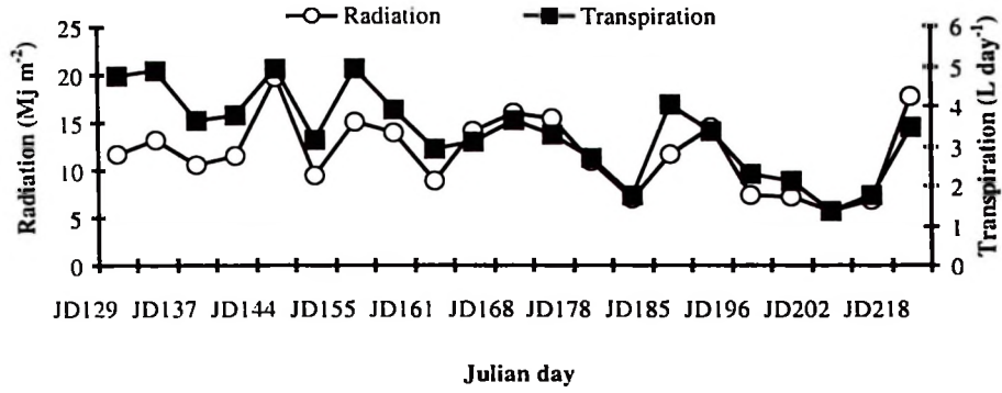
Figure 6.5.3.1 Trends of transpiration rates and solar radiation with time indicating that transpiration rates are influenced by radiation in trial 1 at Machakos.
