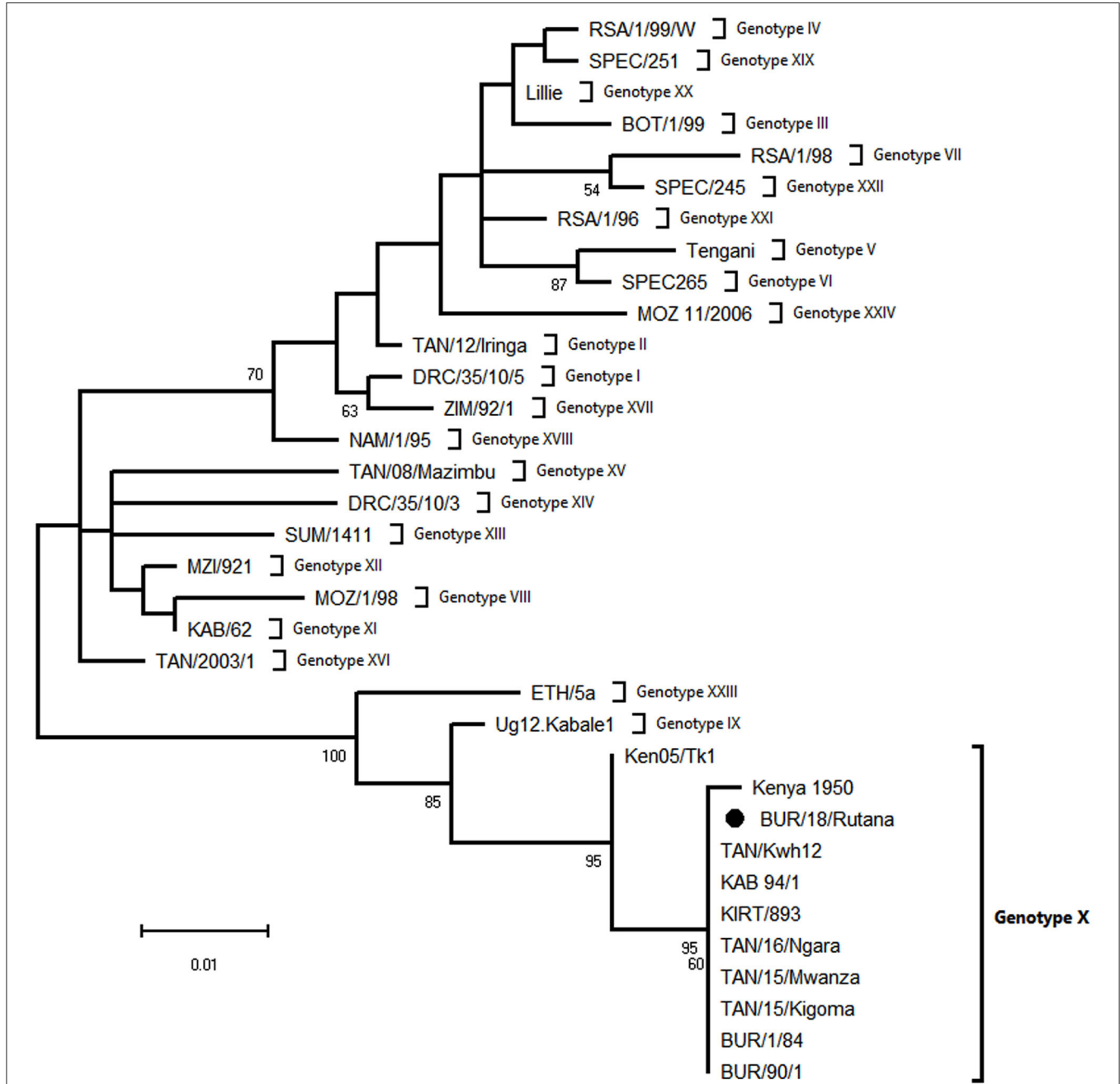
FIGURE 2 | Evolutionary relationships of representative strains of African swine fever virus (ASFV) based on the maximum likelihood phylogeny of the partial p72 gene nucleotide sequences. The phylogenetic analysis was performed using MEGA X ( http://www.megasoftware.net ) and the Kimura two-parameter substitution model, as determined by a model selection analysis. Phylogeny was inferred following 1,000 bootstrap replications, and the node values show percentage bootstrap support (only values above 50% are shown). The round black spot indicates the ASFV nucleotide sequence from Burundi obtained in this study. The scale bar indicates nucleotide substitutions per site.
