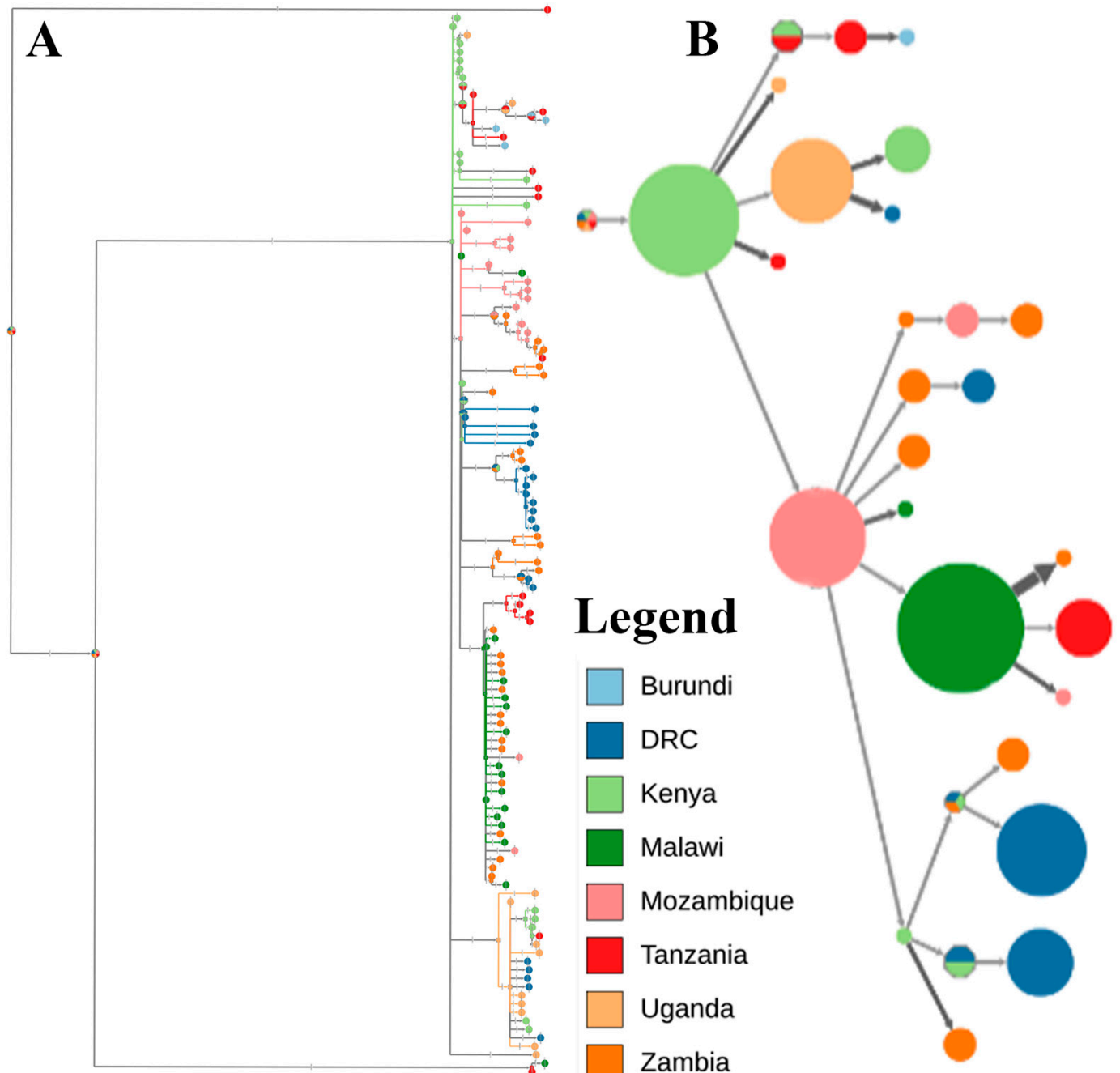
Figure 3. Ancestral reconstruction of African swine fever virus strains collected in Tanzania and its neighboring countries. The figure shows the full tree (A) and compressed (B) visualizations produced by PastML using MPPA with an F81-like model. Different colors correspond to different countries as shown in the legend.
