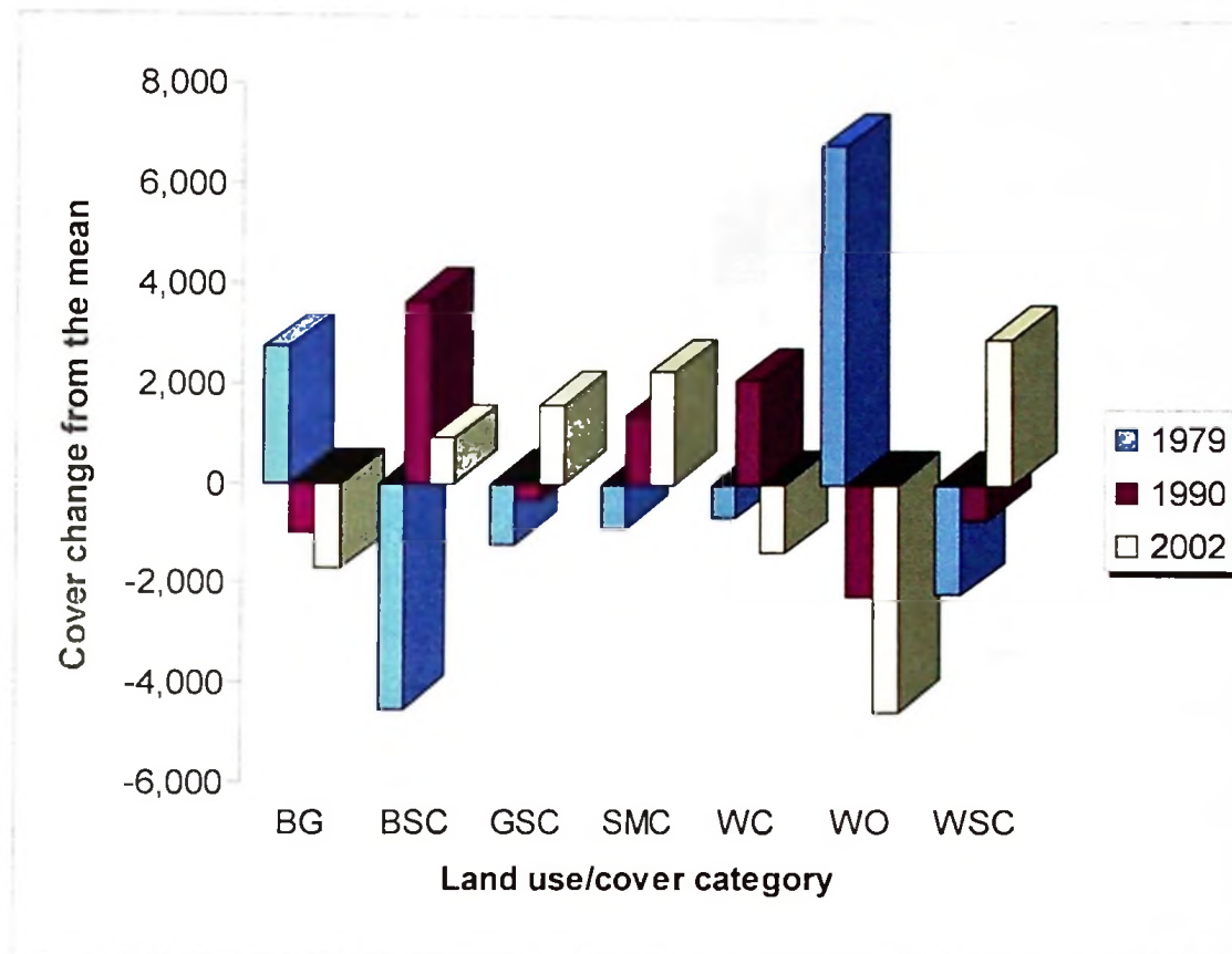
Figure 6: Land use/cover change from the category mean in study area
