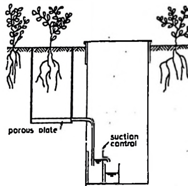
Fig. 3. Non-weighable lysimeter with suction control at the bottom (Kijne, 1980).
