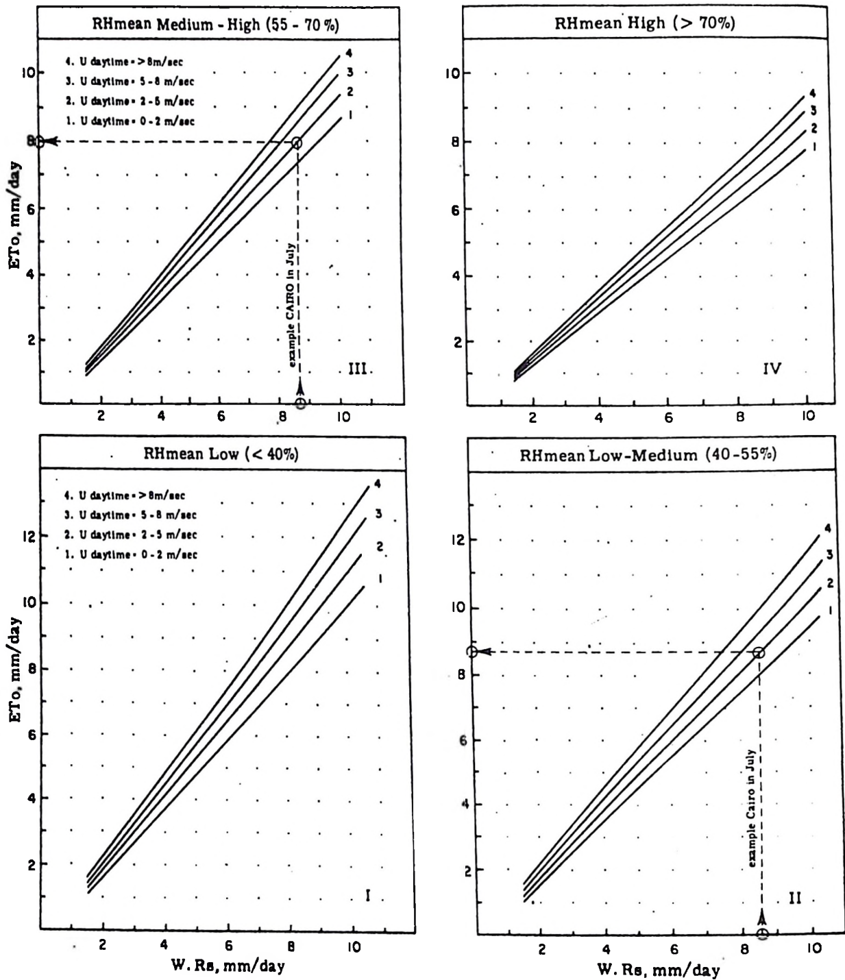
Fig. 6. Prediction of ETo from W x Rs for different conditions of mean relative humidity and daytime wind (Kassam and Doorenbos, 1979).
