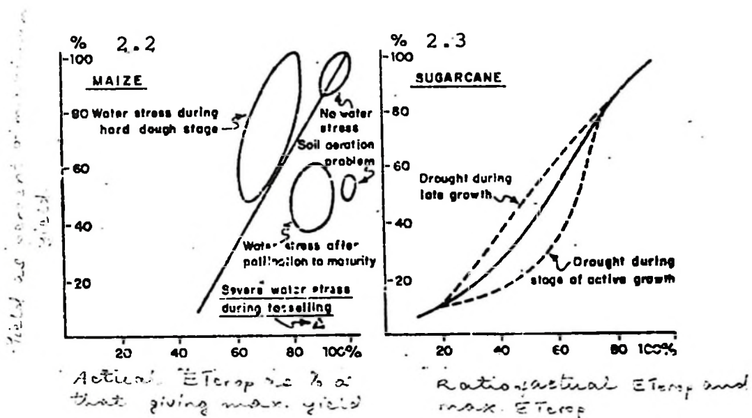
Fig. 2. Relationships between relative yield and relative ETcrop for non-forage crops, corn and virgin cane (Downey, 1972; Chang, 1963).
