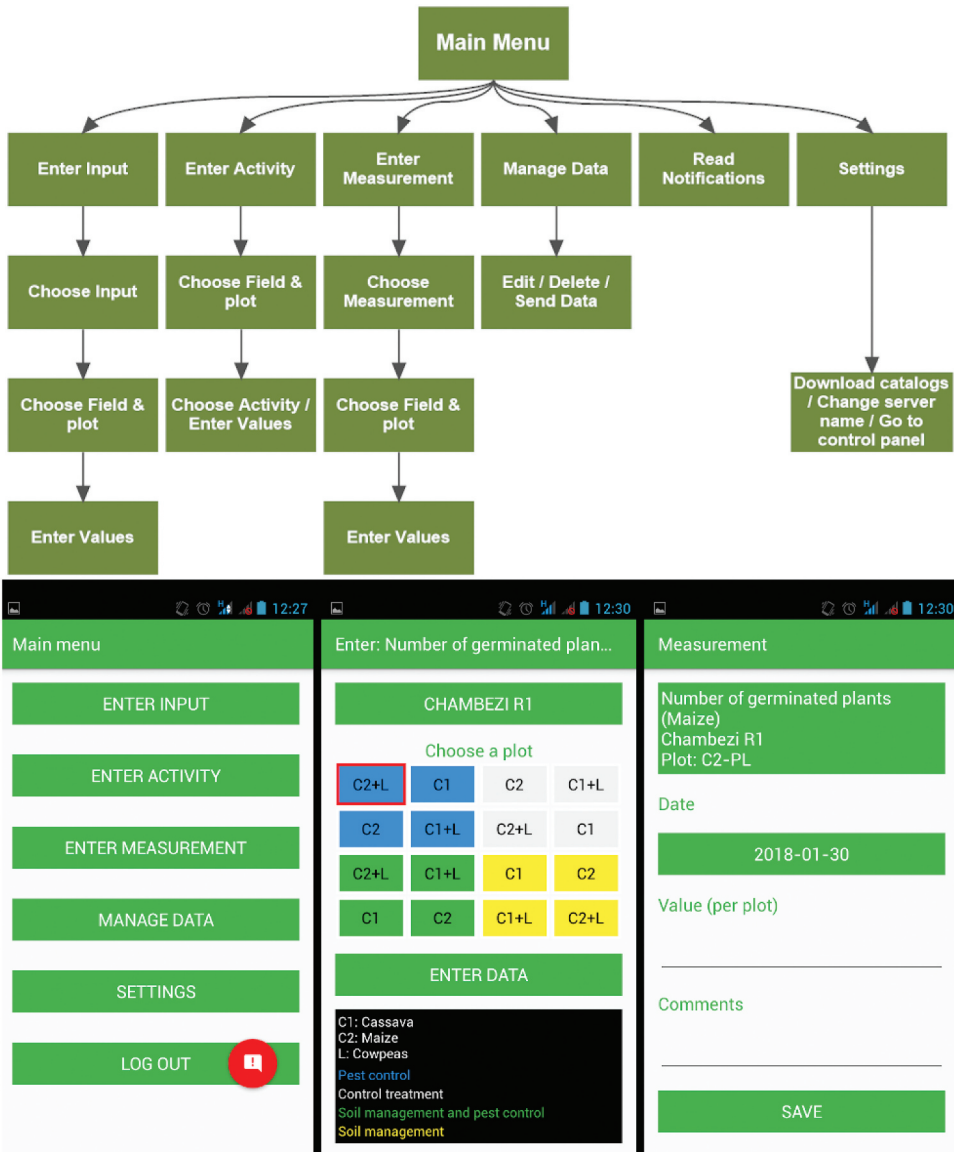
Figure 13. Main navigation diagram and screenshots of the AER mobile application.
