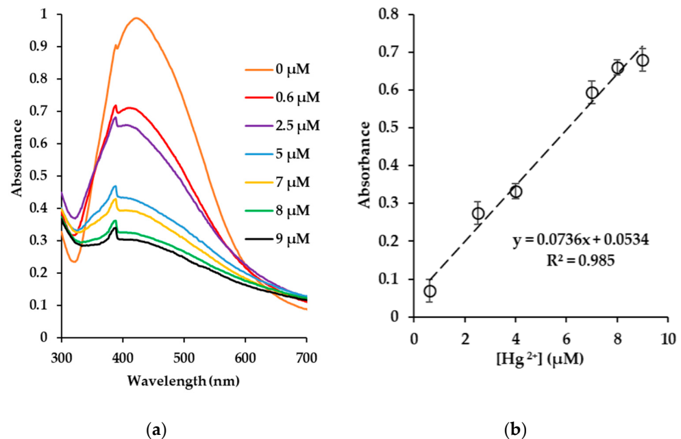
Figure 5. Sensitivity plot (a) and calibration curve (b) prepared for sensing mercury ions in the aqueous sample.
