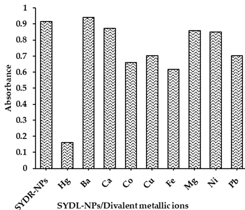
Figure 3. Selectivity of SYDR-AgNPs against various divalent metallic ions.
