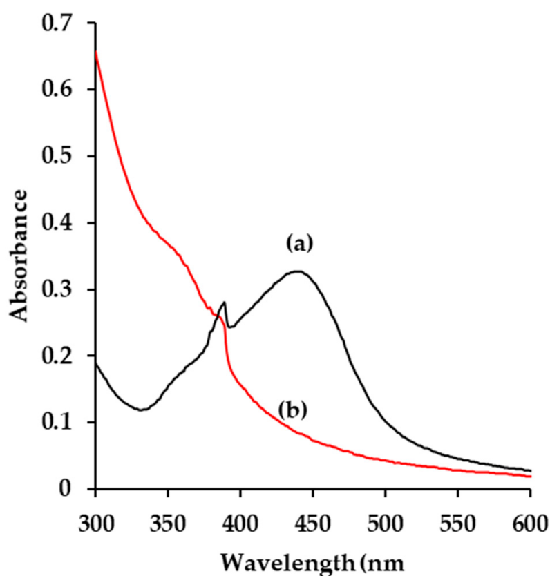
Figure 1. UV-vis spectral of prepared SYDR-AgNPs (a) and SYDR root extract (b).
