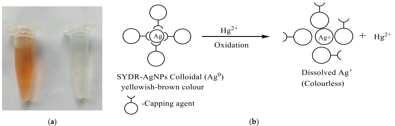
Figure 2. (a) Color change due to the detection of Hg 2+ using fabricated SYDR-AgNPs to produce colorless Hg- SYDR-AgNPs. (b) Schematic illustration of a proposed mechanism for the calorimetric detection of mercury ions using SYDR-AgNPs through a redox reaction.
