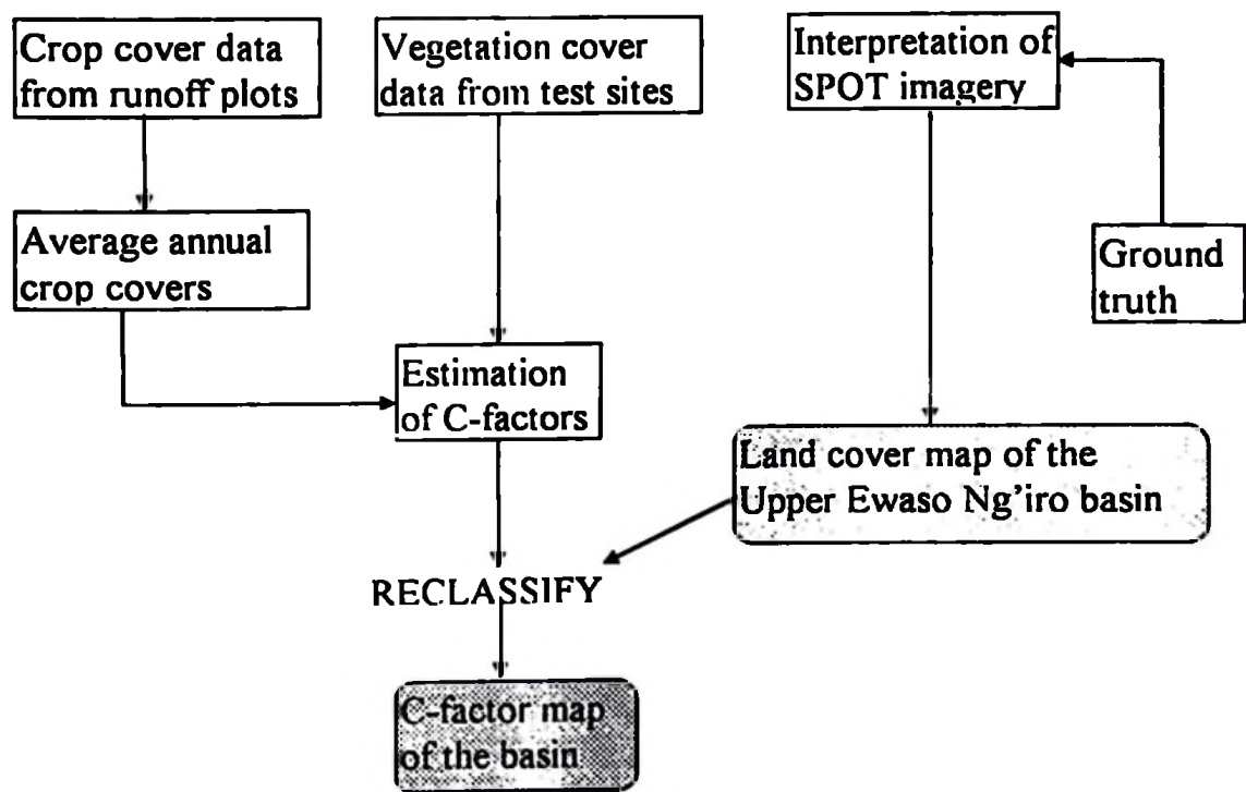
Figure 4.5 Preparation of the land cover and C-factor maps
