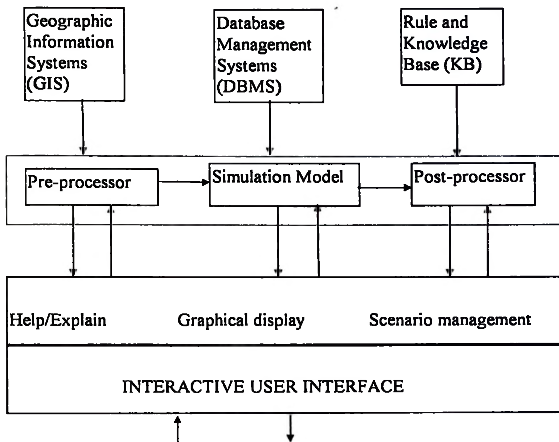
Figure 3.2 Integration of GIS with simulation models (Fedra, 1993)
