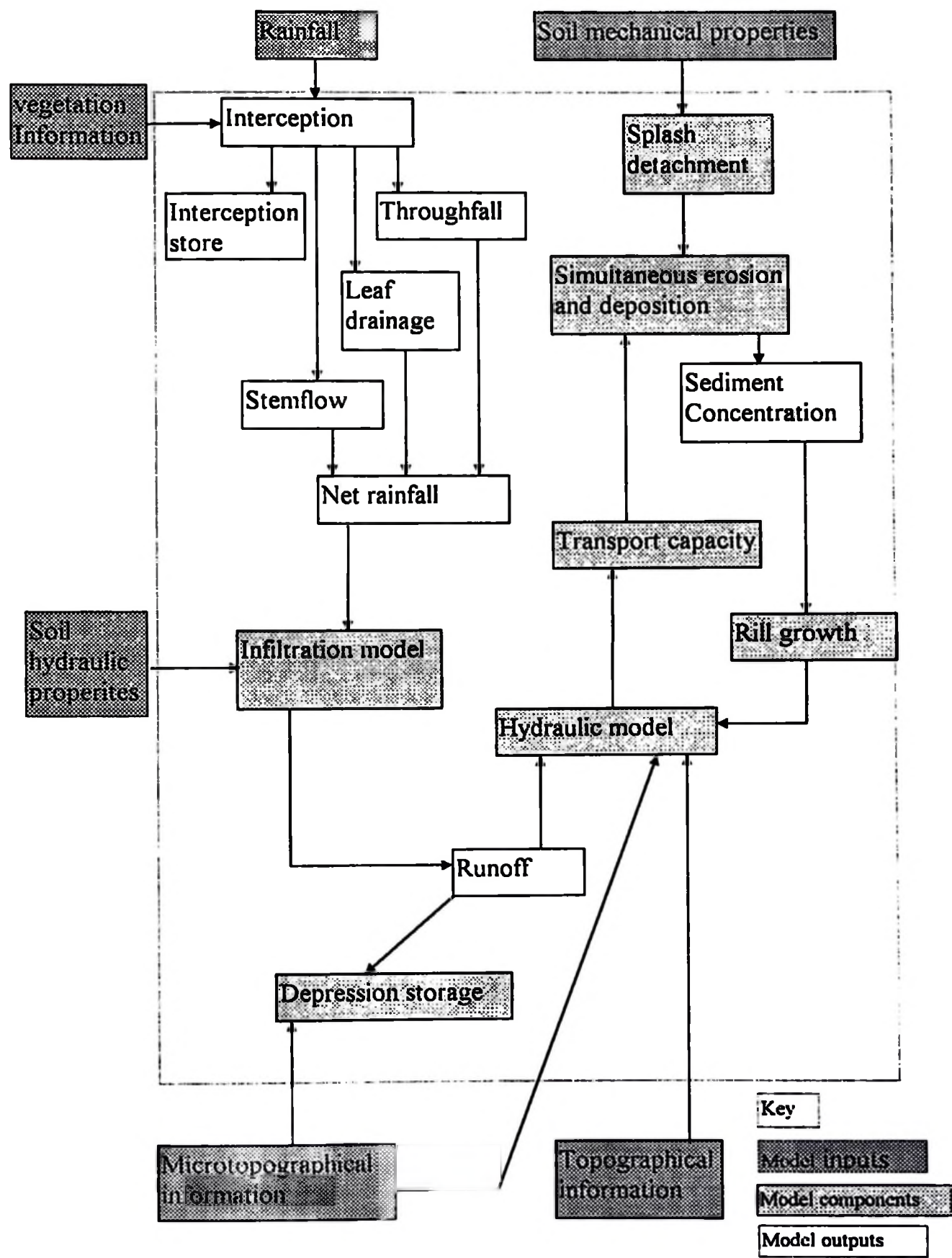
Figure 3.3 Components of EUROSEM (Morgan et al 1998b)
