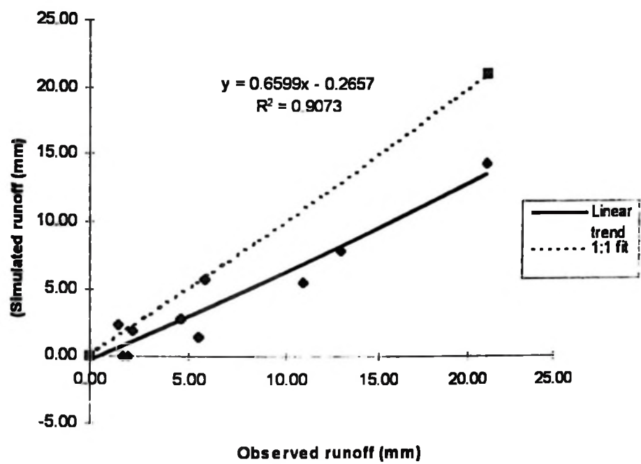
Figure 6.1 Linear regression between observed and simulated runoff for Embori
