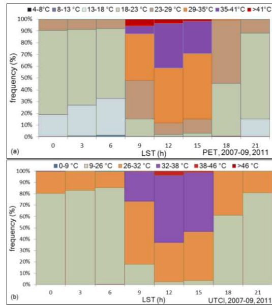
Fig. 5. Diurnal patterns of human thermal bioclimate conditions depicted by (a) PET and (b) UTCI (a, b), using 2007-2009 and 2011 datasets.
