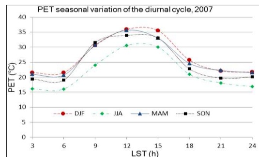
Fig. 6. Diurnal cycle of thermal stress in different seasons of the year, as depicted by PET index.
