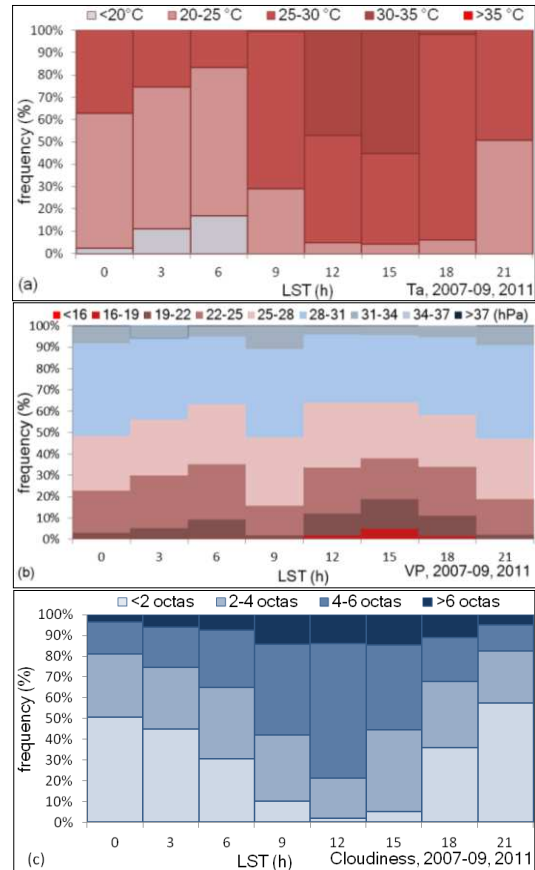
Fig. 3. Frequency of occurrence for the diurnal patterns of air temperature (a), vapour pressure (b) and cloudiness (c) for 2007-09 and 2011 data.
