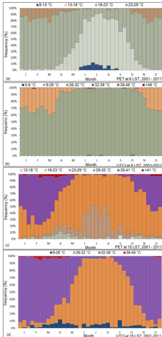
Fig.4. Annual patterns of human thermal bioclimate conditions as depicted by PET and UTCI indices at 6 LST (a, b) and at 15 LST (c, d).
