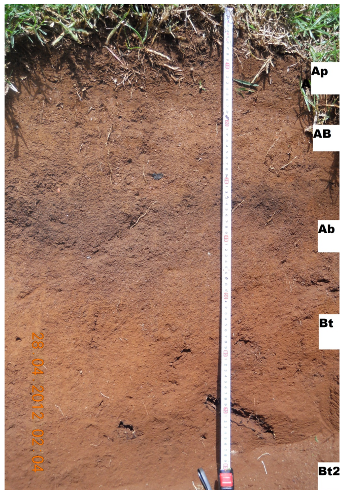
Profile 1 Typical profile of a Luvis Ferralic Phaeozem on backslopes and footslopes in the Lukozi area
