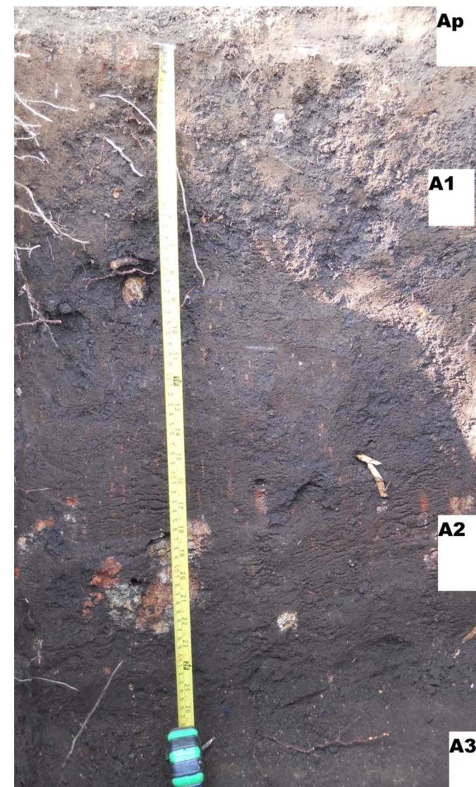
Profile 3 Haplic Leptic Cambisol (colluvic, eutric, skeletic, humic) on an escarpment in Nywelo village
