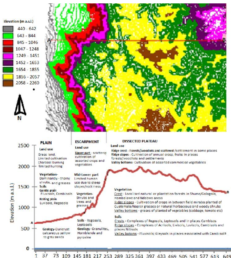
Figure 1: Major landform characteristics of the study area
