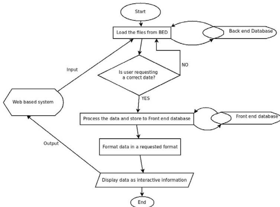
Figure 1: ECAWsoft flowchart
