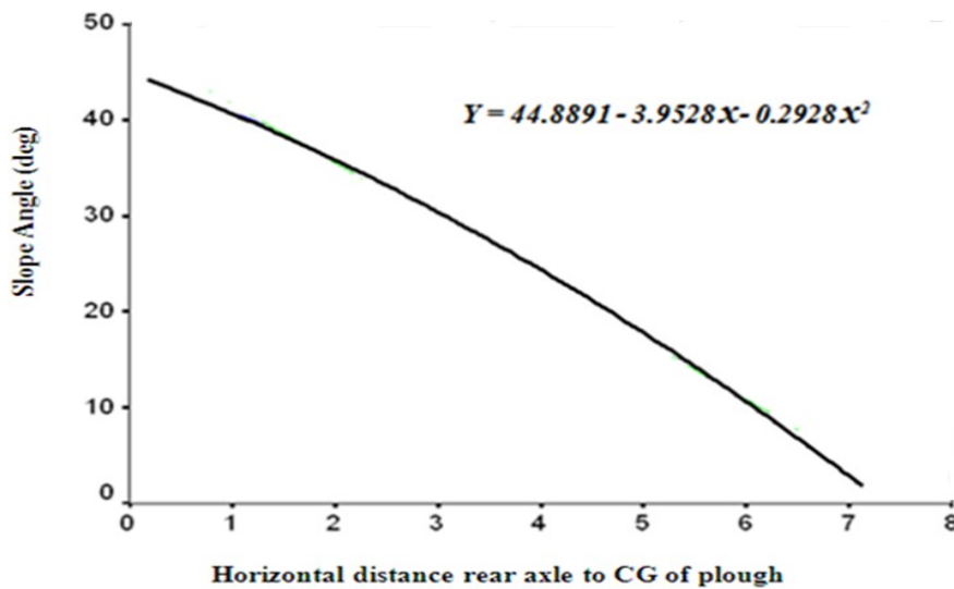
Figure 29: Maximum operating slope angles ( \beta ) Vs Horizontal dimension from rear axle to centre of gravity of mounted plough
