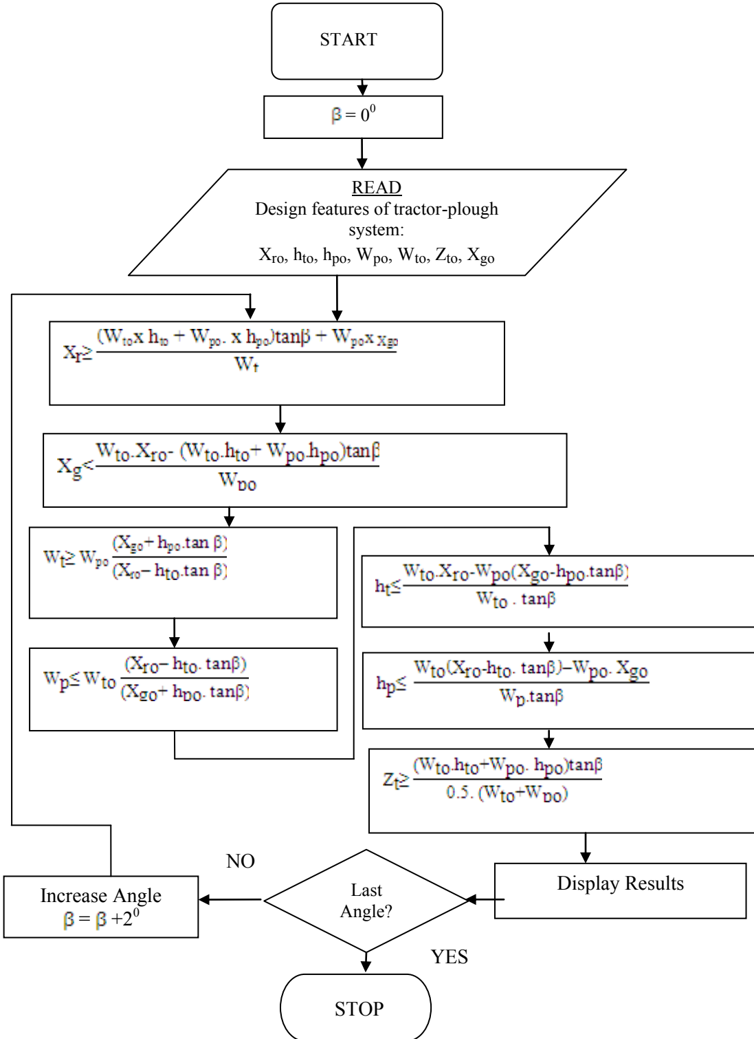
Figure 18: Flow chart of static stability simulation program.
