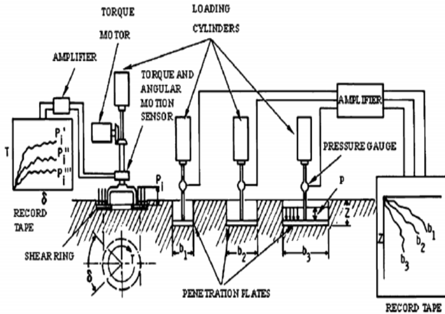
Figure 3: Schematic layout of a bevameter (Wong, 1993).
