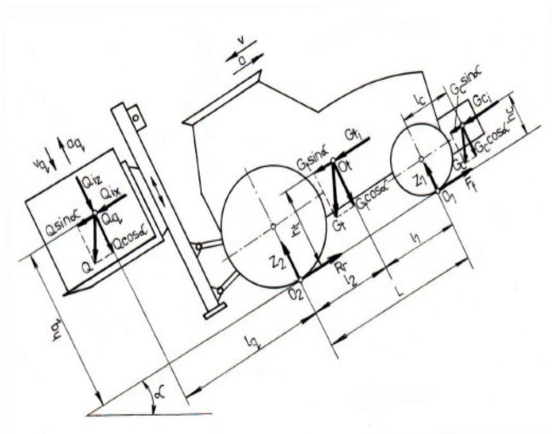
Figure 13: Forces acting on the tractor- forklift system operating on sloping road (Simion and Nastase, 2009).
