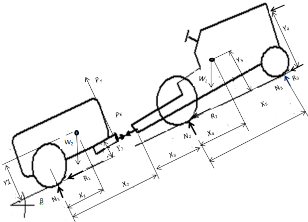
Figure 11: Schematic of representation of forces acting on tractor-trailer system (Abu-Hamdeh and Al-Jalil, 2004).
