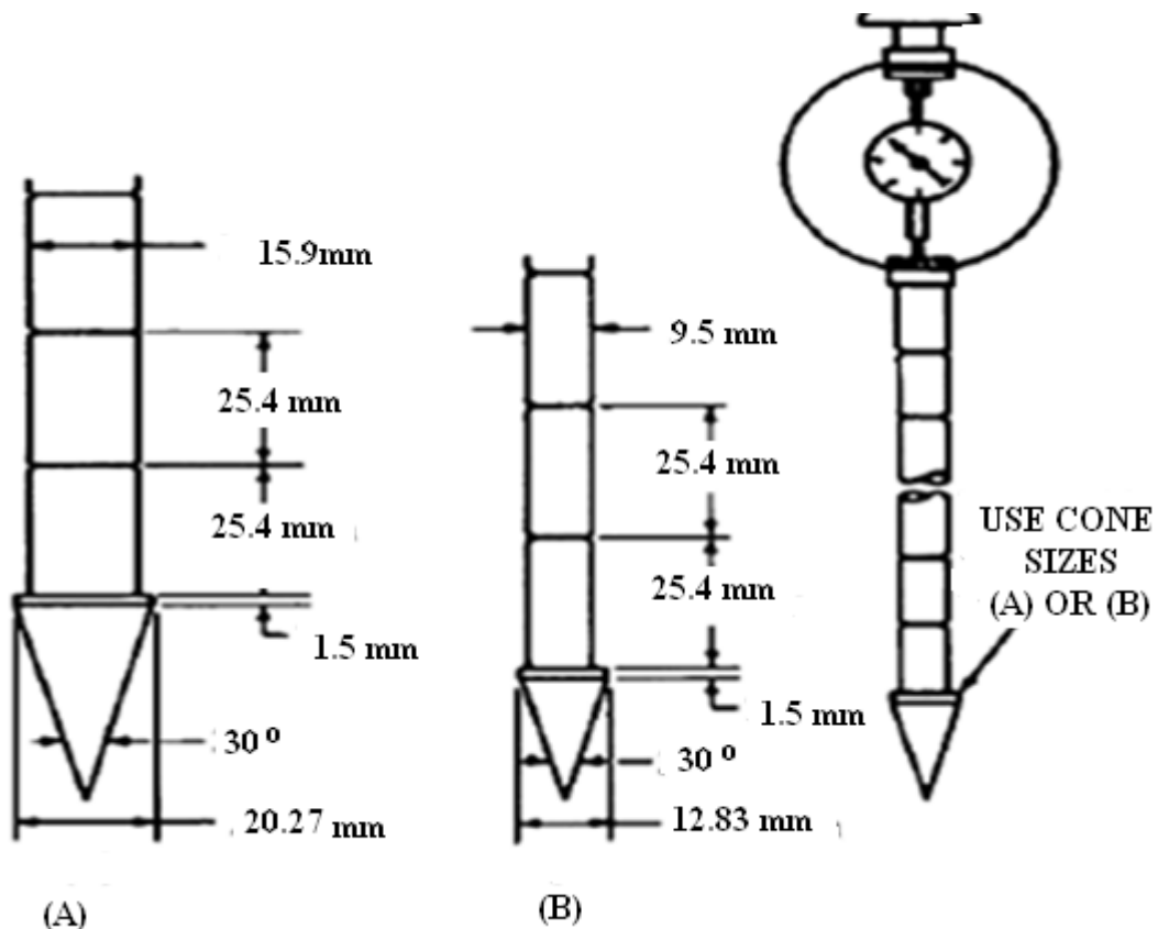
Figure 4: Cone penetrometer (ASAE, 1998).
