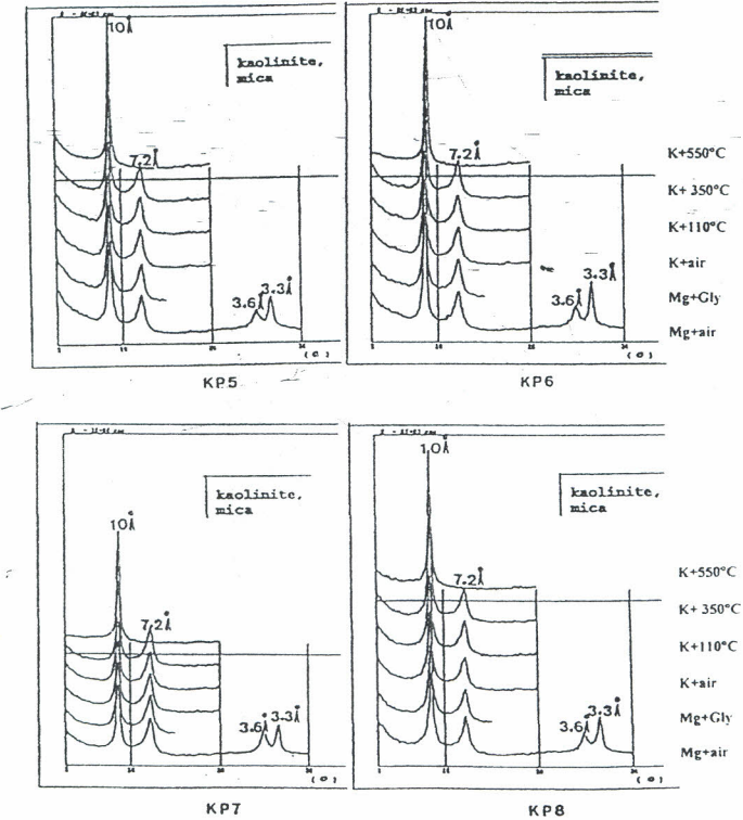
Figure 2: X-ray diffractograms of subsoil clay fractions of the soils of Mikese Area, Morogoro
